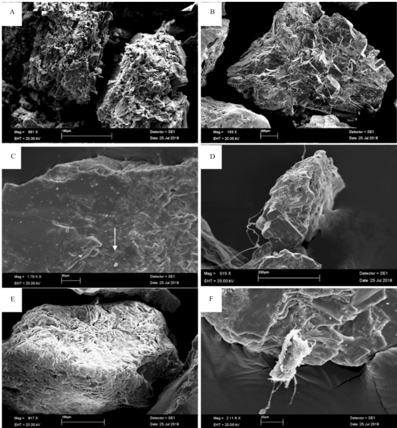
Figure 2. Scanning electron microscopy images of remineralizer (RM) grains, showing: A and B, fine and coarse sand fraction of the grains of the RM used as a control (RM-control), respectively; C, etched pits and a crack probably caused by mechanical stress during comminution (arrow) in the coarse sand fraction of the RM after being buried for 154 days in soil cultivated with corn ( Zea mays ); D, cleavage surfaces (possibly of a feldspar) and biological filament entangled to it in the fine sand fraction in the RM after being buried for 378 days in soil with elephant grass ( Pennisetum purpureum ); E, rounded surfaces, possibly due to preferential edge dissolution in the fine sand fraction in the RM after being buried for 378 days in soil in the woods, contrasting with the coarse sand fraction of the RM-control; and F, biological structure (possibly biofilm) at the edge of the grain, whose corrosion seems more intense around the biological structure in the coarse sand fraction in the RM after being buried for 378 days in the woods.
