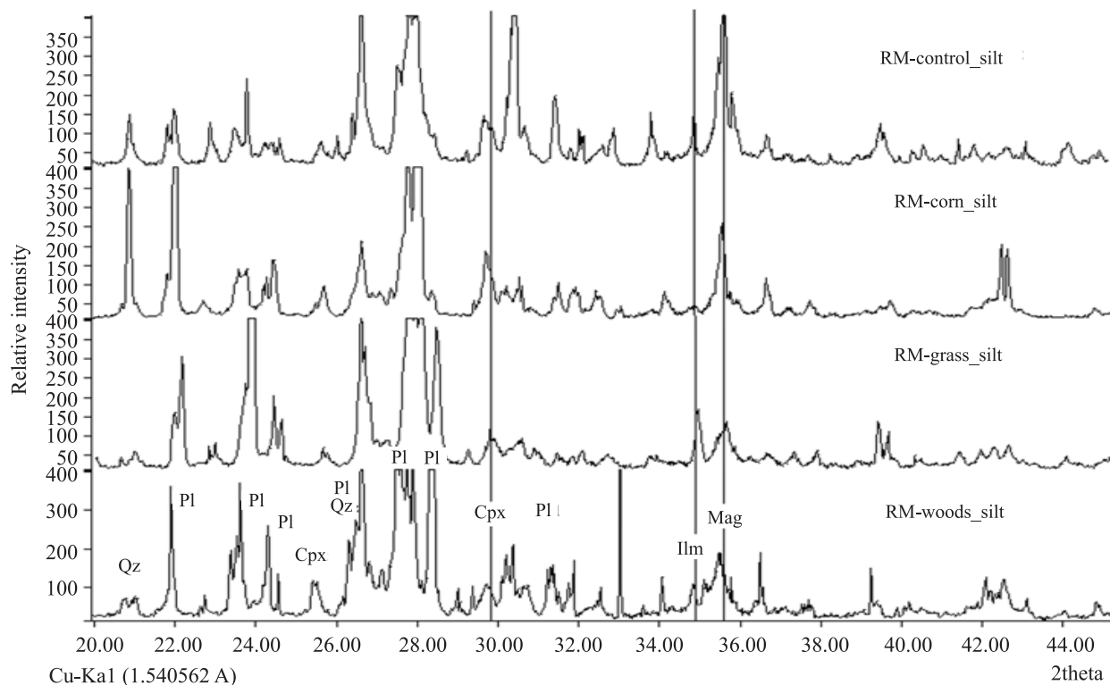
Figure 5. X-ray diffraction scans of the silt fraction of the remineralizer used as a control (RM-control), after being buried for 154 days in soil cultivated with corn ( Zea mays ) (RM-corn) and for 378 days in soil under elephant grass ( Pennisetum purpureum ) (RM-grass) and woods (RM-woods). Qz, quartz; Pl, plagioclase; Cpx, clinopyroxenes; Ilm, ilmenite; and Mag, magnetite.
