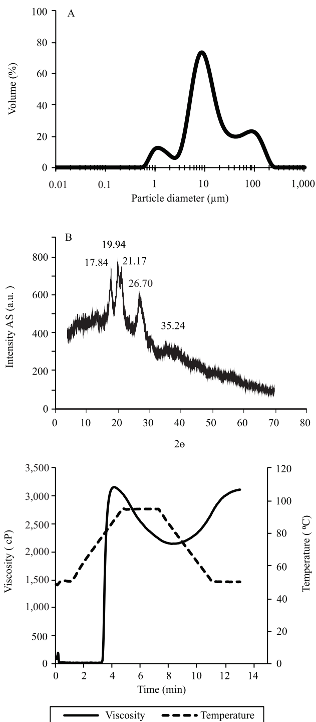
Figure 2. Distribution of the size of the granules of Xanthosoma riedelianum starch (A); X-ray diffractogram of the starch (B); and suspension viscoamylographic profile (10% p/v) of the starch (C).
