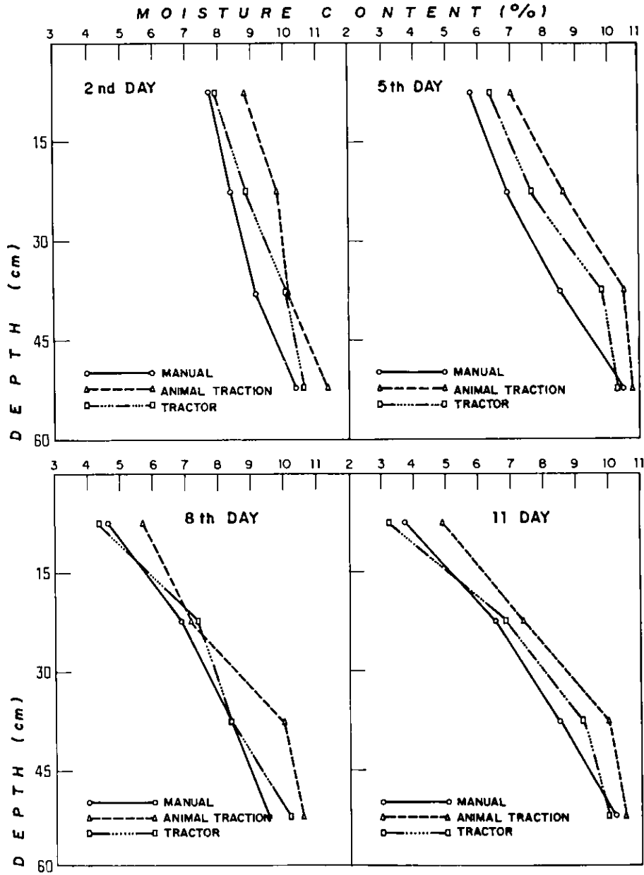
FIG. 3b. Soil moisture content in various layers on various days after irrigation as affected by different methods of soil preparation.
