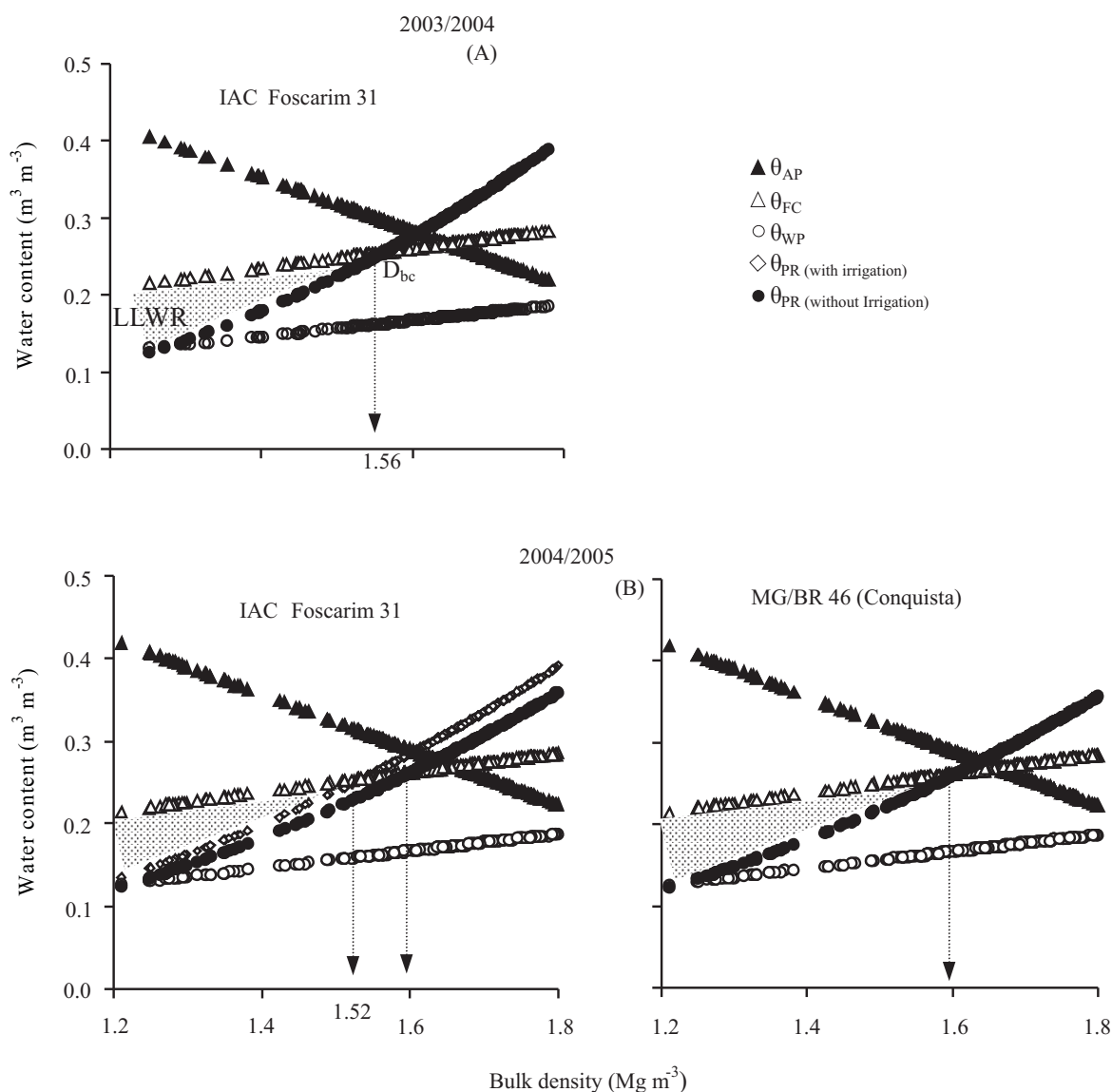
Figure 3. Variation of water content ( \theta ) with D_b to critical limits of aeration porosity ( \theta_{AP} ), field capacity ( \theta_{FC} ), soil penetration resistance ( \theta_{PR} ) and permanent wilting point ( \theta_{WP} ), in 2003/2004 (A) and 2004/2005 (B), at 0.0–0.20 m depth. LLWR, least limiting water range; D_{bc} , critical soil bulk density.
